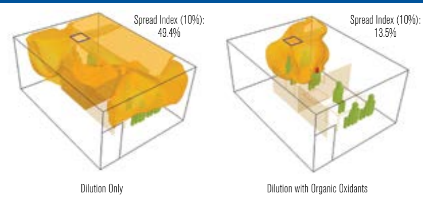
FIGURE 6 Impact of organic oxidants on the Spread Index of probability of infection ( SI_{10} ) indicating the extent of the space volume at or above the 10% infection probability—ach: 3 h -1 .
