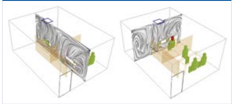
FIGURE 3 Airflow patterns in an office space showing large recirculation zones.
