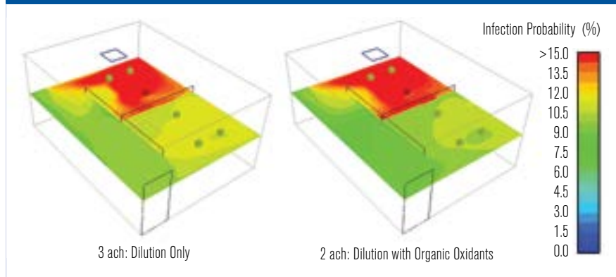
FIGURE 7 Impact of organic oxidants with reduced ach 2 h -1 on the distribution of infection probability at the breathing zone at 4.5 ft (1.4 m) from the floor.
