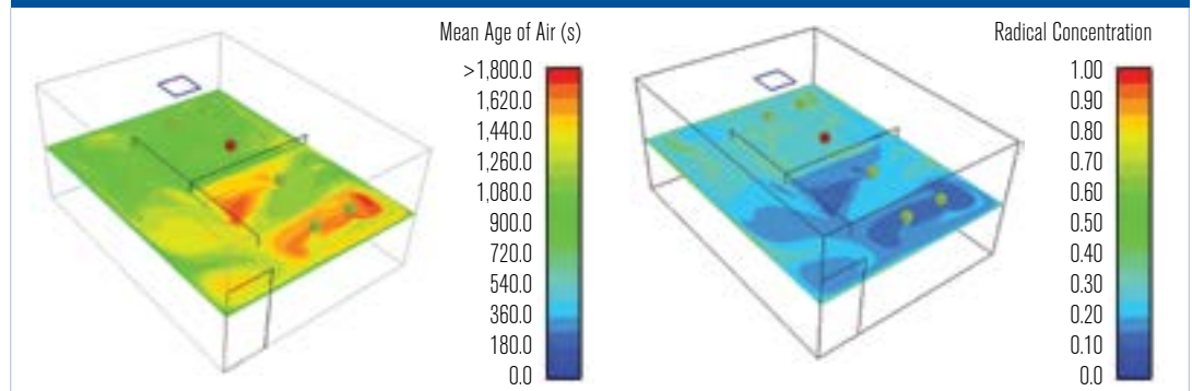
FIGURE 4 Age of air (s) and resulting radical concentration at a breathing plane at 4.5 ft (1.4 m) from the floor.
