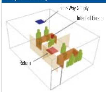
FIGURE 2 Schematic of the office CFD model analyzed in this study.
